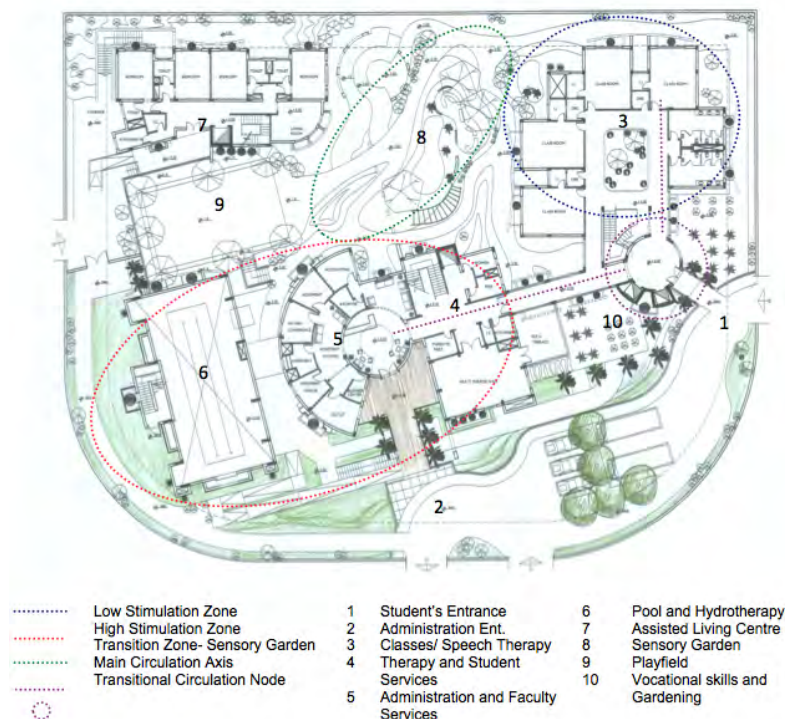
Figure 3: Entry-level plan and Sensory Zoning (Source: Author).
